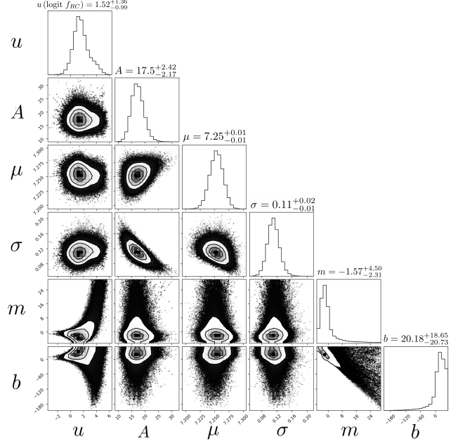
Figure 6. Corner plot of the MCMC posterior for NRCB1 F115W-F212N versus F115W (tile k = 3 ).
