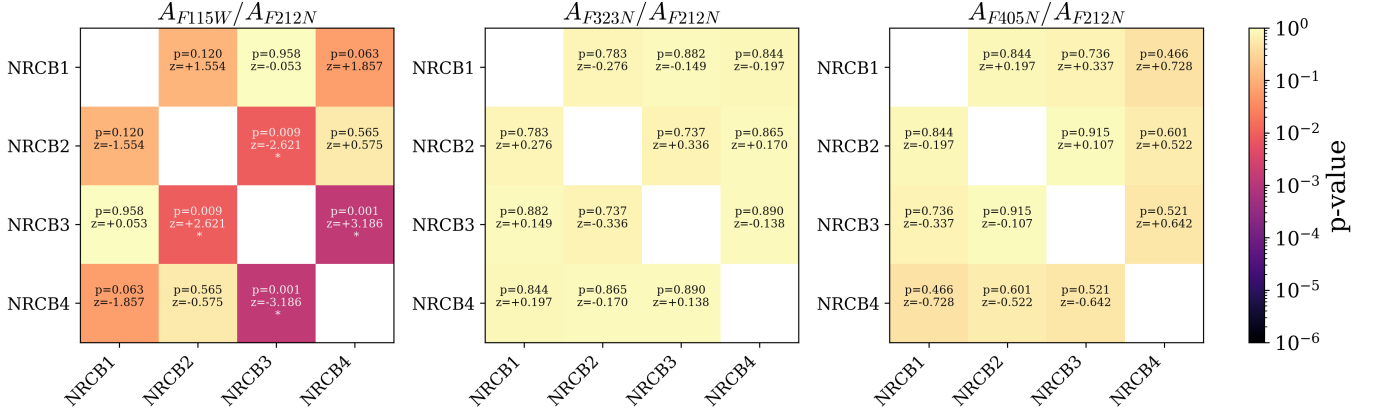
Figure 10. Heatmaps of pairwise p -values (log scale) and Z -scores comparing extinction ratios A_\lambda/A_{F212N} across NRCB1–4. Asterisks mark p < 0.05 ; darker cells indicate higher significance.
