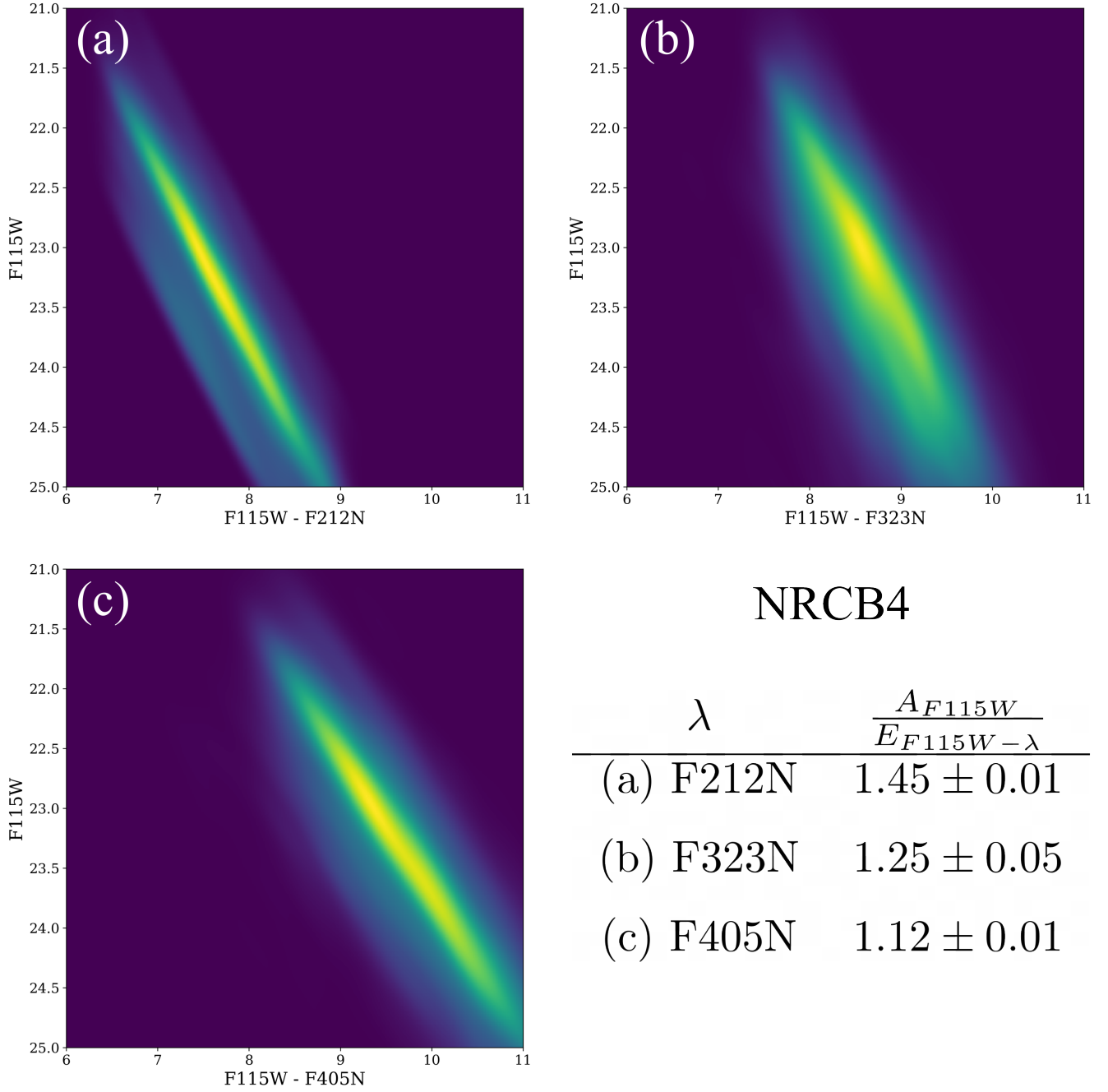
Figure 15. The Red Clump stars in the NRCB4 footprint: (a) F115W–F212N vs. F115W, (b) F115W–F323N vs. F115W, and (c) F115W–F405N vs. F115W. The overdensities trace the RC sequence, and the measured slopes were used to estimate the ratios of total to selective extinction, reported in the bottom-right quadrant. The RC stars were selected following the procedure described in Section 3.2.
