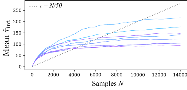
Figure 5. Integrated autocorrelation time \hat{\tau}_{\text{int}} as a function of total samples N for 8/10 CMD tiles from NRCB1 F115W - F212N vs. F115W that satisfied Equation 4. Each colored curve tracks the mean autocorrelation across all sampled parameters in one tile. The black dashed line denotes the heuristic convergence criterion \tau = N/50 . Curves that flatten below the dashed line by N \approx 10^4 indicate that the 15000 step runs achieve an effective number of independent samples sufficient for reliable posterior estimation.
