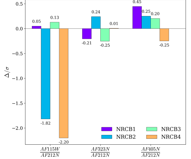
Figure 9. Total extinction A_\lambda significance relative to Fritz et al. (2011) across all NRCB footprints.
