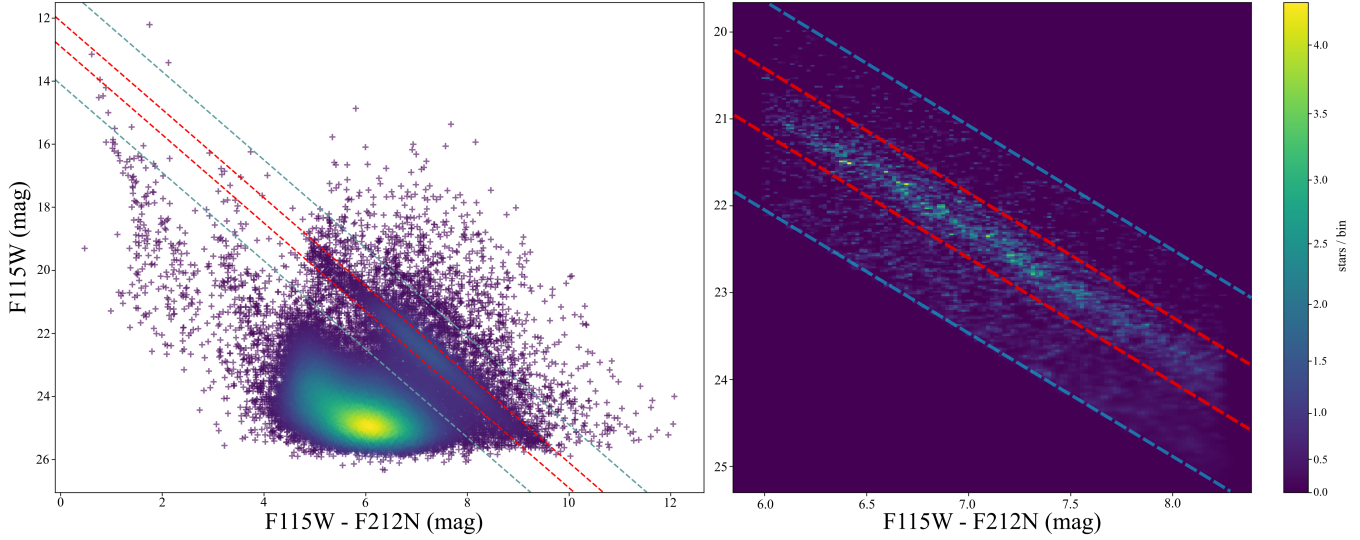
Figure 2. Selection of RC stars in NRCB1. Following De Marchi et al. (2016), the observed CMD (left panel) is converted into a Hess diagram and unsharp masking is applied to isolate the high-density RC ridge; initial by-eye boundaries (red lines) are then drawn around this feature and expanded by a factor of three (blue lines) to ensure comprehensive RC star coverage.
