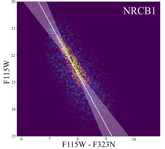
Figure 11. Left: Overview of the algorithm used to measure the RC ridge slope in CMDs where the RC is broad or poorly defined. Right: Application of Method 2 to the F115W-F323N versus F115W CMD. The f_{\text{top}} = 0.4 highest-density stars are overplotted on the unsharp masked Hess diagram; the white line shows the best fit linear slope from the MCMC posterior, and the shaded band shows the uncertainty envelope obtained from N = 500 \pm \epsilon \sim 30\% jitter Monte Carlo MCMC sweeps. This cross-check is used only for the F115W-F323N versus F115W CMDs for all NRCB footprints.
