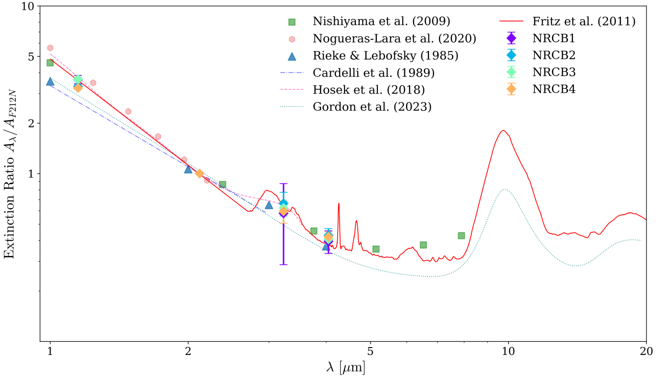
Figure 7. Discrete near-infrared extinction measurements for all NRCB 60'' \times 60'' footprints in the Galactic Center. The red solid curve shows the Fritz et al. (2011) GC extinction law (NRCB3), the dashed pink line shows the Hosek et al. (2018) GC extinction law, green squares mark the Nishiyama et al. (2009) law, blue triangles denote the Rieke & Lebofsky (1985) law, and pink hexagons show the Nogueras-Lara et al. (2020) law. The dashed blue and dotted teal lines indicate the diffuse Milky Way ISM laws of Cardelli et al. (1989) and Gordon et al. (2023) , respectively. Laws were rendered using SPISEA ( Hosek et al. 2020 ).
