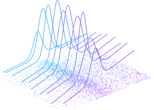
Figure 4. Three-dimensional view of the NRCB1 red clump ridge analysis with n = 10 tiles. The fitted Gaussian means from each tile trace out the RC ridge in this rotated frame.
