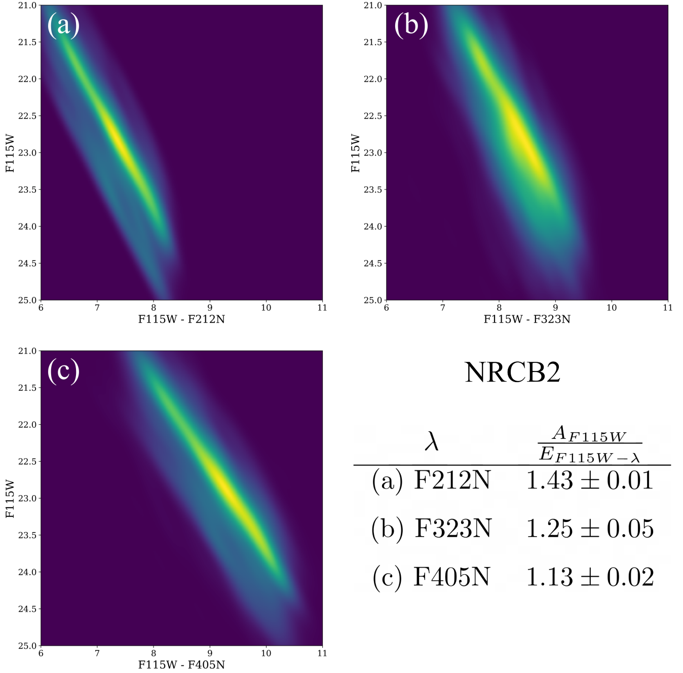
Figure 13. The Red Clump stars in the NRCB2 footprint: (a) F115W–F212N vs. F115W, (b) F115W–F323N vs. F115W, and (c) F115W–F405N vs. F115W. The overdensities trace the RC sequence, and the measured slopes were used to estimate the ratios of total to selective extinction, reported in the bottom-right quadrant. The RC stars were selected following the procedure described in Section 3.2.
