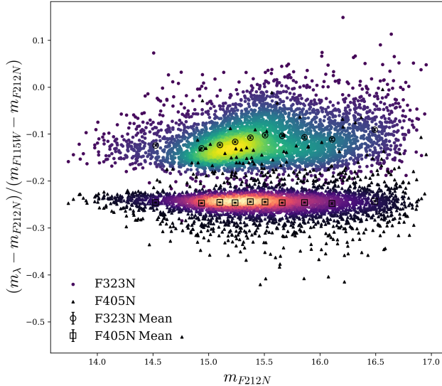
Figure 8. Extinction ratio vs. Total Extinction proxy for NRCB1. RC stars are plotted as F323N circles and F405N triangles. The horizontal axis m_{F212N} traces total extinction A_{F212N} , while the vertical axis y_\lambda = (m_\lambda - m_{F212N}) / (m_{F115W} - m_{F212N}) encodes A_\lambda/A_{F212N} . The near-horizontal trends in all NRCB footprints show that the extinction ratios at 3.23 \mu\text{m} and 4.05 \mu\text{m} are roughly independent of column density.
