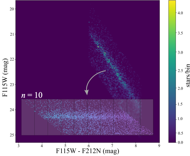
Figure 3. Method 1 – Tiles are generated along the RC bar to guide the collective MCMC slope fit: the CMD is first rotated by an angle \theta = \tan^{-1}(m_{\text{ansatz}}) to horizontalize the RC ridge, then n = 10 vertical bins are placed across this rotated ridge, and MCMC is used to fit a compound Gaussian + linear model in each tile (Figure 4).
