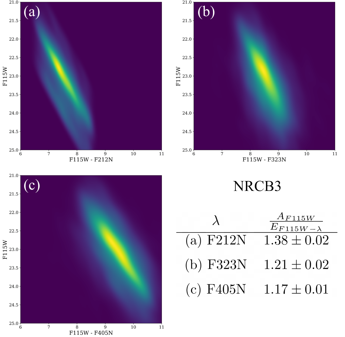
Figure 14. The Red Clump stars in the NRCB3 footprint: (a) F115W–F212N vs. F115W, (b) F115W–F323N vs. F115W, and (c) F115W–F405N vs. F115W. The overdensities trace the RC sequence, and the measured slopes were used to estimate the ratios of total to selective extinction, reported in the bottom-right quadrant. The RC stars were selected following the procedure described in Section 3.2.
