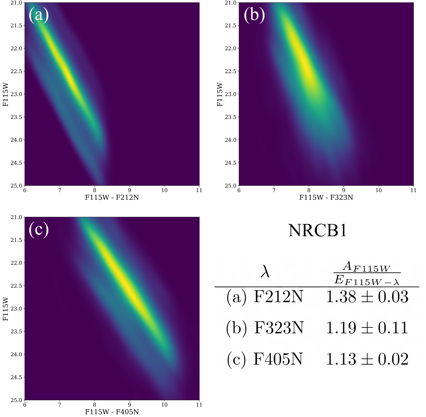
Figure 12. The Red Clump stars in the NRCB1 footprint: (a) F115W–F212N vs. F115W, (b) F115W–F323N vs. F115W, and (c) F115W–F405N vs. F115W. The overdensities trace the RC sequence, and the measured slopes were used to estimate the ratios of total to selective extinction, reported in the bottom-right quadrant. The RC stars were selected following the procedure described in Section 3.2.
